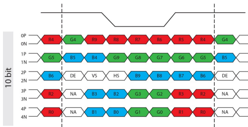
JEIDA Format (LVDS)
