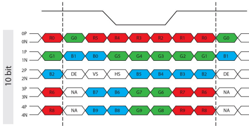
VESA Format (LVDS) (Mapping A)
